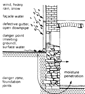
⑥ Main points of attack by non-pressurised water
